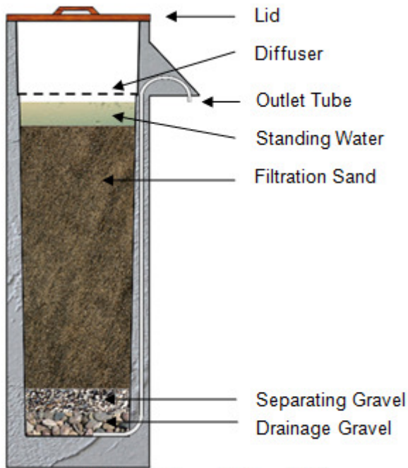
Cross-Section of Concrete Biosand Filter
