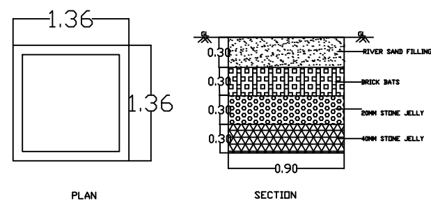
RAIN WATER HARVESTING PLAN (FILTER UNIT) SECTION NOT TO SCALE
